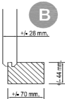
Shinglesdak Schindeldach Shingleroof
