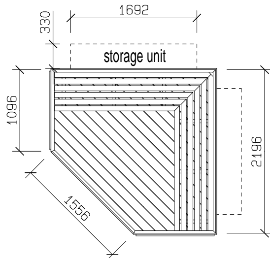
TOP VIEW, SHOWN WITHOUT ROOF
